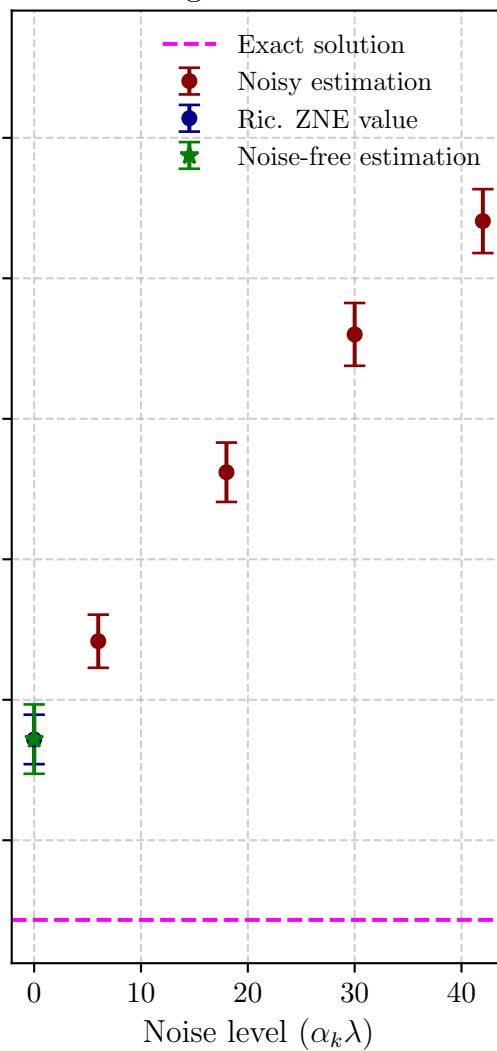
Ising ansatz ric-4
